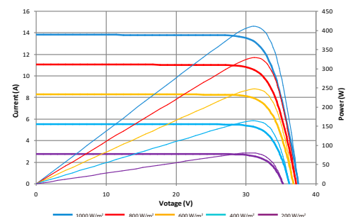
Current-Voltage & Power-Voltage Curve (410)
